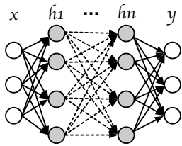
Figure 1: DNN architecture
