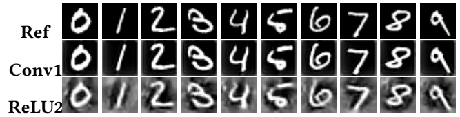
(a) MNIST.
