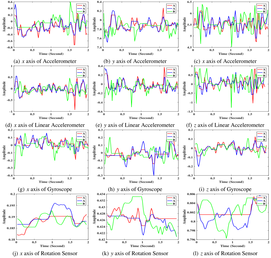
Figure 1: The visualization of handwritten signals extracted from the accelerometer, linear accelerometer, gyroscope and rotation sensor under the three different dimensions. We randomly select two handwritten signals from the same character A (red and blue lines) and a handwritten signal from another character B (green lines). We observe that the distance between two handwritten signals corresponding to the same character is smaller than that from a different character, which lays the foundation of our attack.
