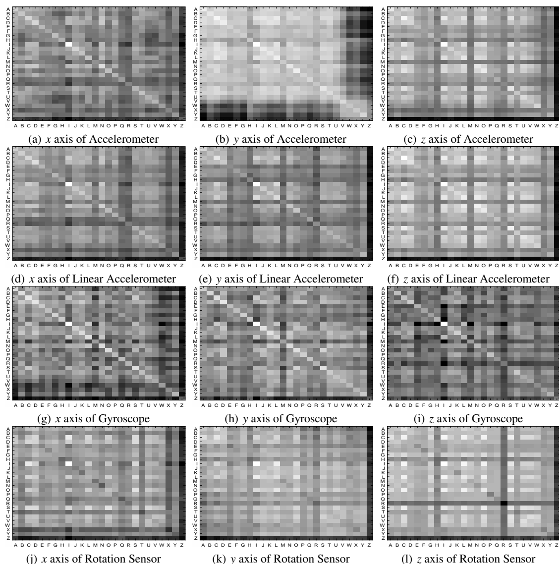
Figure 2: The heatmap of DTW distance between sensor measurements corresponding to any pair of characters from A to Z by using different dimensions of motion sensors (the accelerometer, linear accelerometer, gyroscope and rotation sensor). A whiter color corresponds to a smaller DTW distance between two characters. We observe various distinguishing powers of motion sensors in differentiating users' handwritten patterns.
