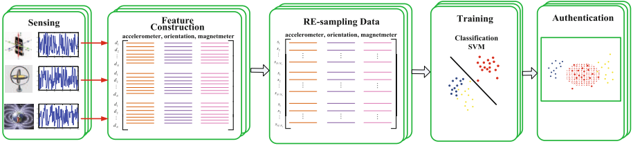
Fig. 1. In our method, we first construct a vector at each sample time by using sensors’ data. For example, our three-sensor-based method uses 9 values from the accelerometer, magnetometer and orientation sensor in a smartphone. After that, we re-sample the data collected from the sensors. Then, we train the re-sampled data with the SVM technique to get a user’s profile. Based on the user’s profile, we can do the implicit authentication.
